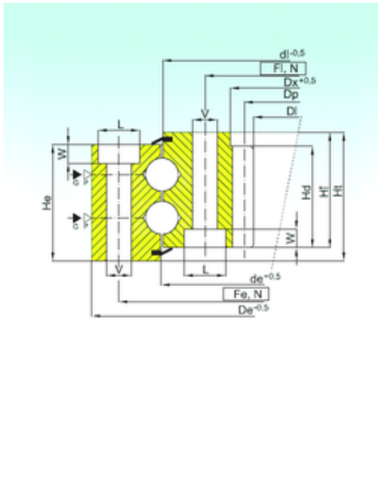
ZB2.30.1613.400-1SPPN Bearing 2D drawings and 3D CAD models
