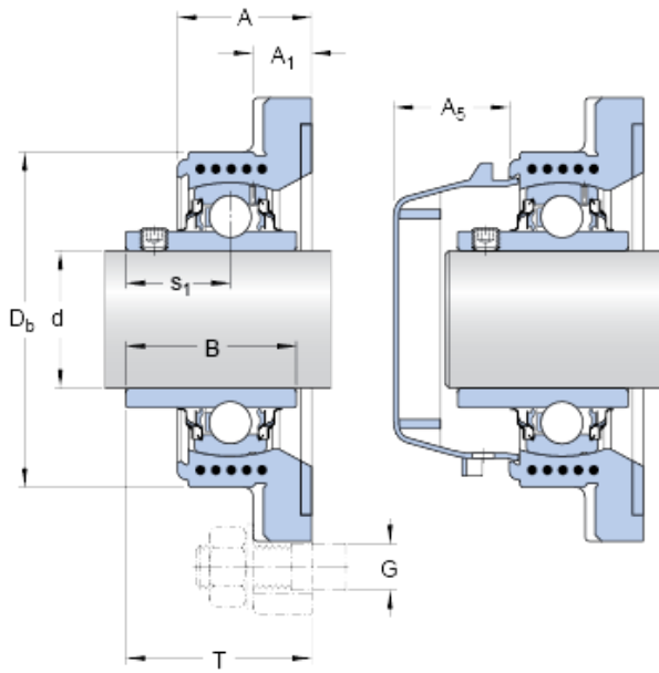
Bearing No. FYWK 25 YTH
