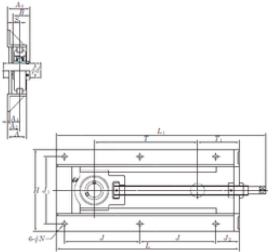
Bearing No. UCTH205-150
