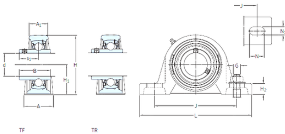
Bearing No. SY 50 TF
